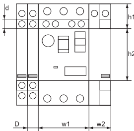
Auxiliary contact UVR
